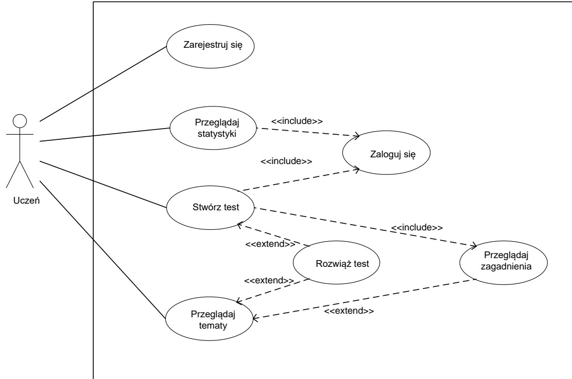
Figure 5: Use case diagram – Service to Learner
