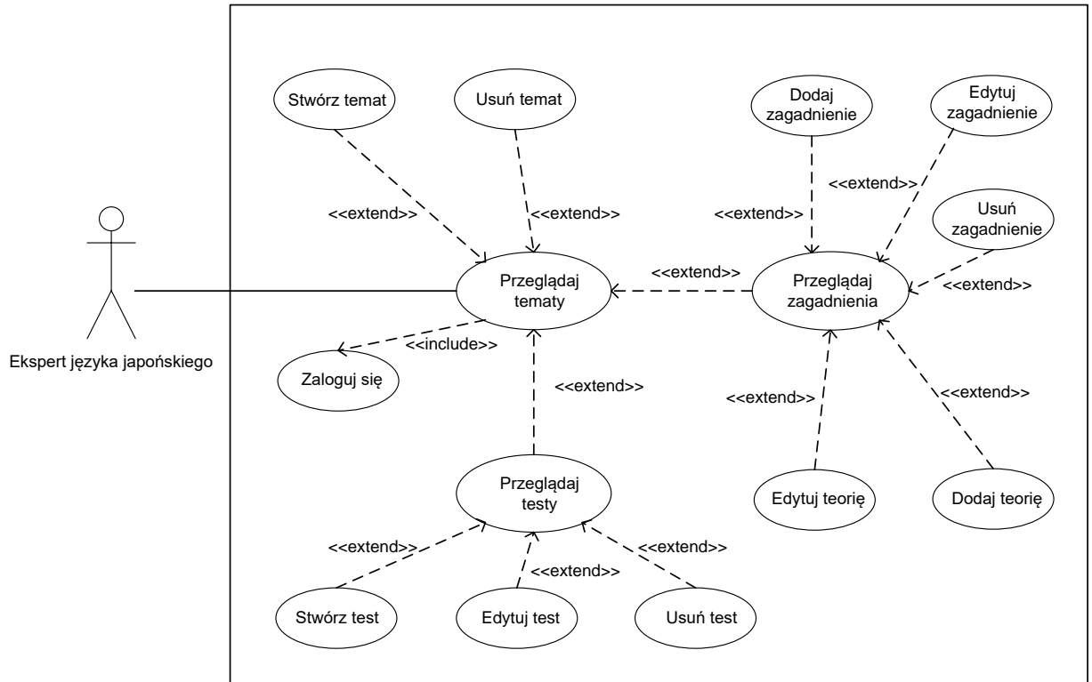
Rysunek 4: Figure 4. Use case diagram - Service of the database of topics
