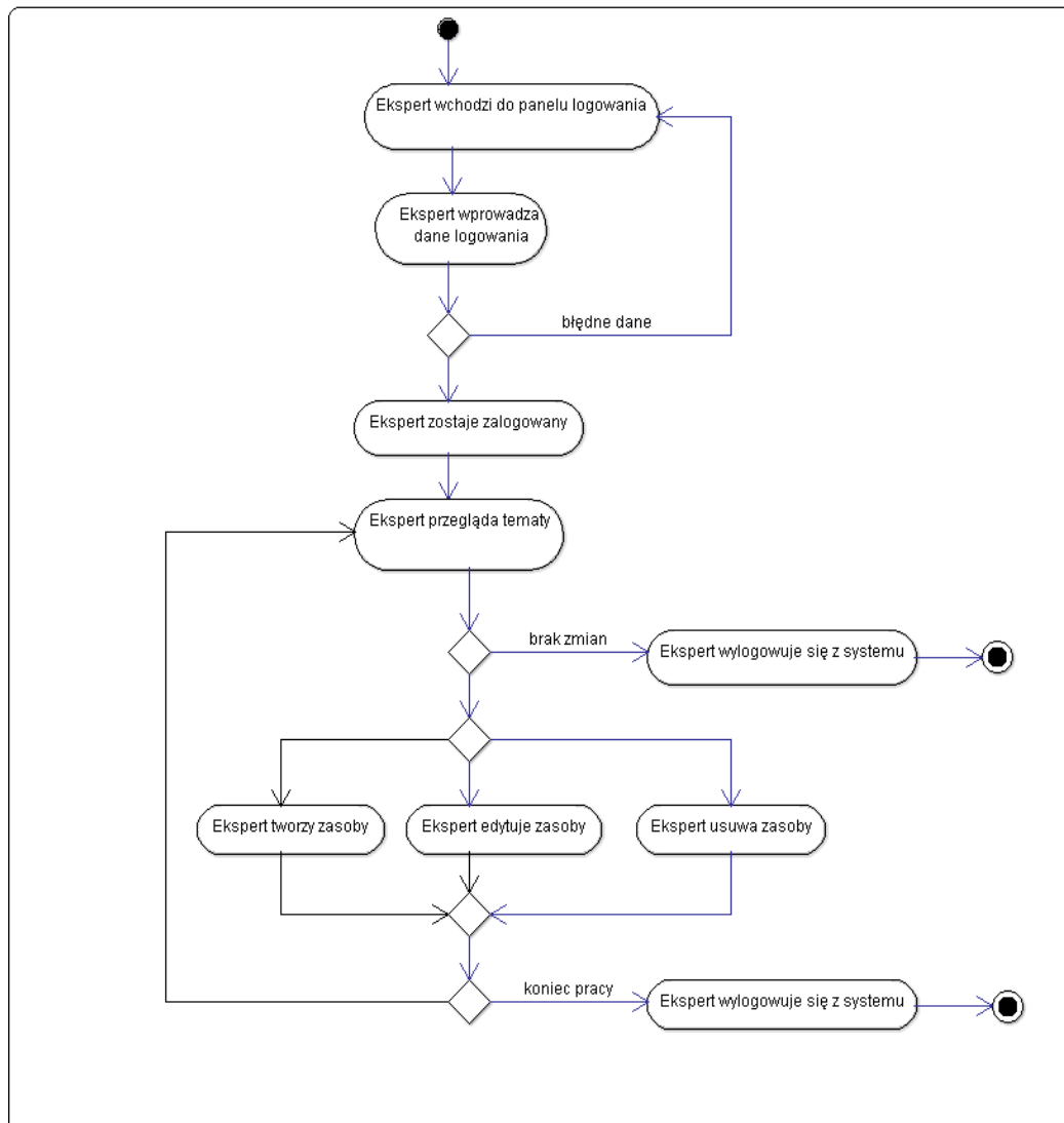
Figure 6: Activity diagram for the user/expert
